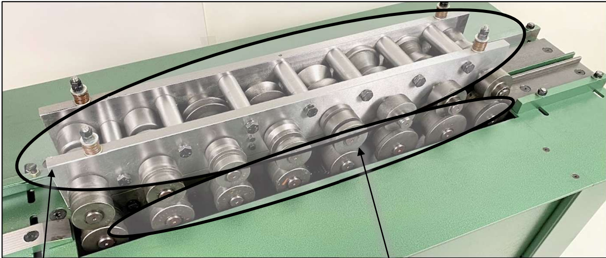
Top Assembly (see p. 3)
