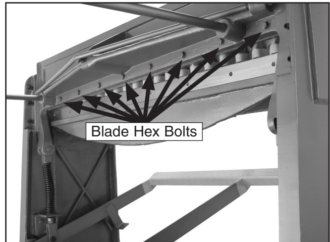
Figure 31. Blade bolts.
