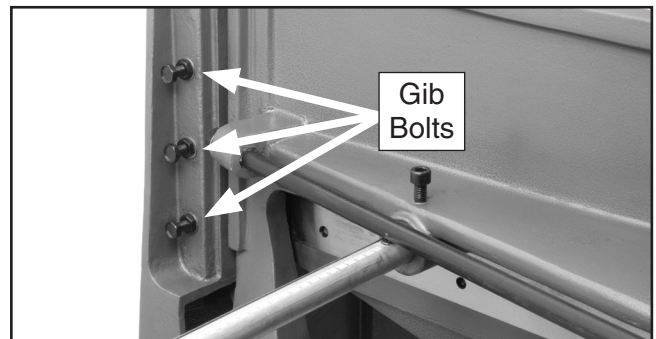
Figure 34. Gib bolt location.
