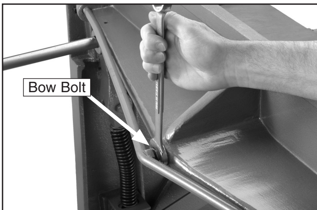
Figure 33. Adjusting bow bolt.
