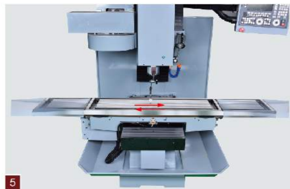
5 Parallelism of the T slot and X axis movement is also an inspection value. Normally per 40" the tolerated maximum number is 0.0008".
