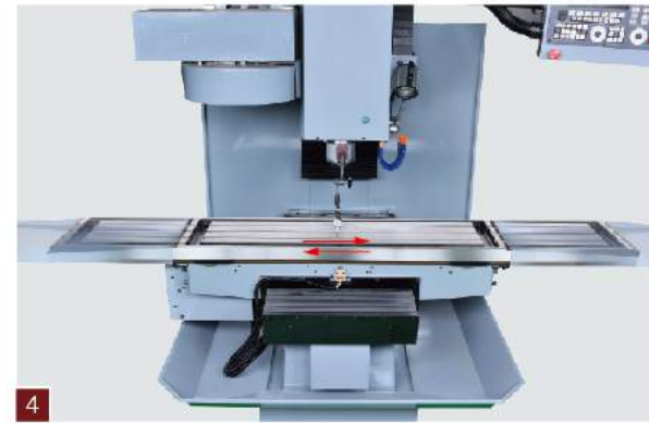
4 Parallelism of the table movement in X axis is dial in with a dial indicator. The permissible value is 0.0004" per 20".
